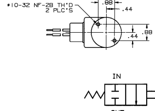
Port Identification: 1-OUT/ 2-IN
