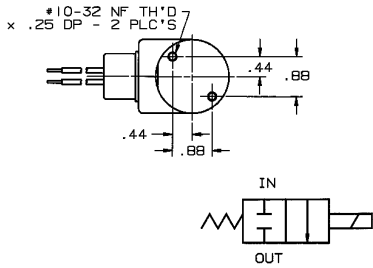
Port Identification: 1-OUT/ 2-IN
