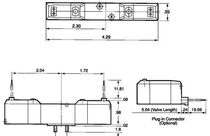
K5R valve
