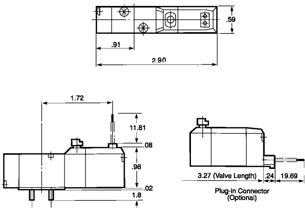
K4RL valve
