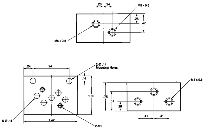
KR-01-001 subbase
