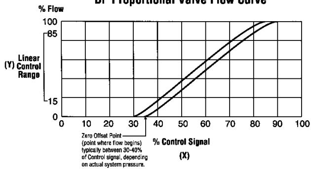
BP Proportional Valve Flow Curve
