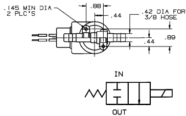
Port Identification: Flow area on body indicates flow direction—ports are not marked.
