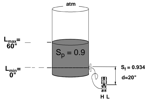
FIGURE 1. Open tank, single seal system, transmitter below the tap
