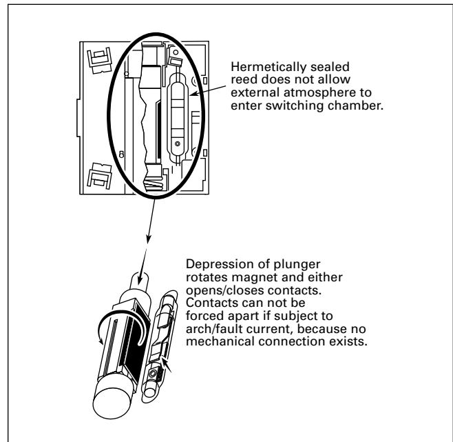
Figure 47-149. Hermetically Sealed Reed Contact Block
