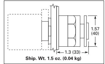
Figure 47-49. E22/EM22 Series 3-Position 40 mm Dia. Lens (Spring Return to Center)
