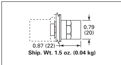
Figure 47-57. E22/EM22 Series 2-Position — 60° Throw — Knob
