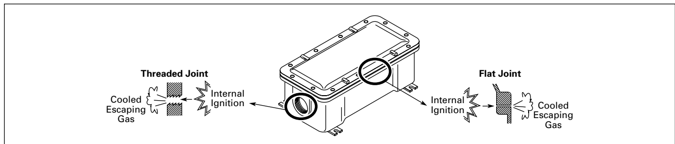
Figure 47-150. Explosion Proof Enclosure
