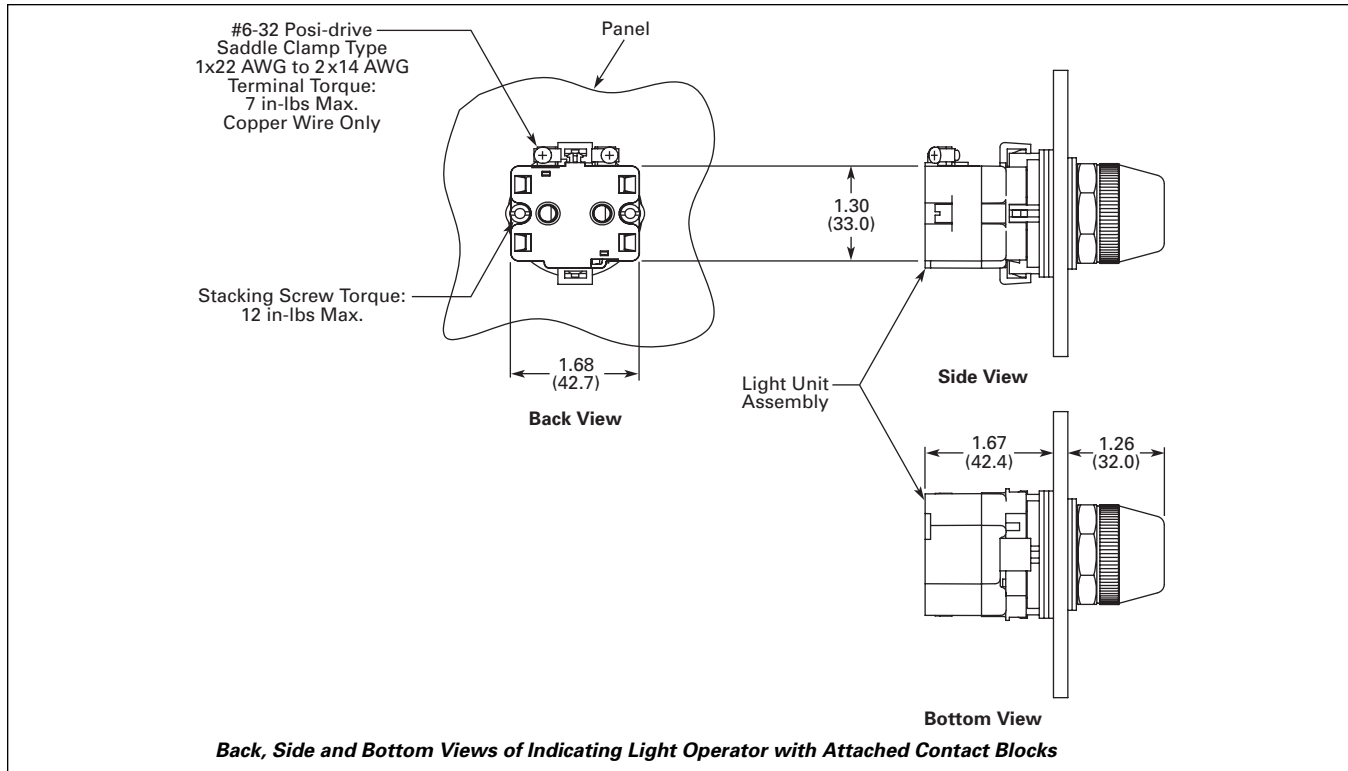
Figure 47-133. Indicating Lights — Approximate Dimensions in Inches (mm)
