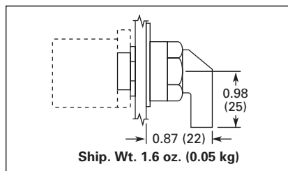
Figure 47-60. E22 Series 2-Position — 45° Throw — Lever
