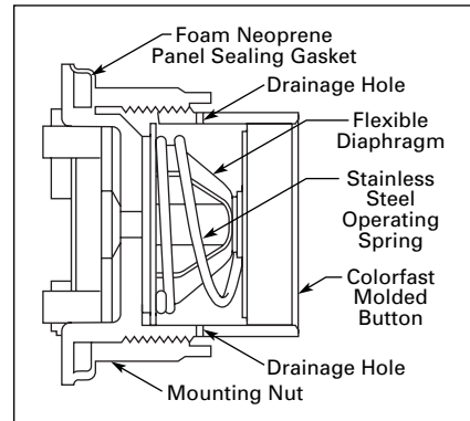
Figure 47-116. Diaphragm Seal
