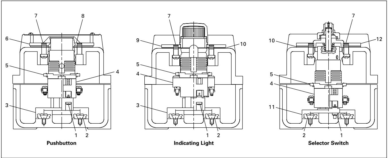
Figure 47-8. Type H Renewal Parts
