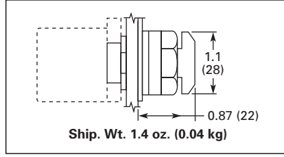
Figure 47-24. E22/EM22 Series 28 mm Dia. Mushroom Head Button
