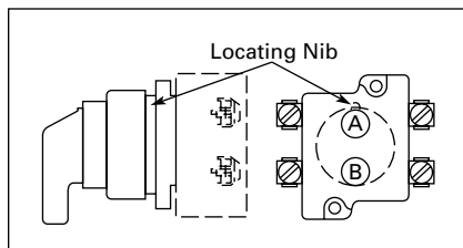
Figure 47-118. Contact Circuit Locations
