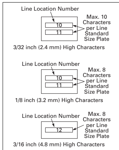
Figure 47-16. Insert Type Plates
