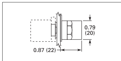
Figure 47-63. E22 Series 3-Position — 60° Throw — Knob
