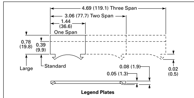
Figure 47-81. Approximate Dimensions in Inches (mm)
