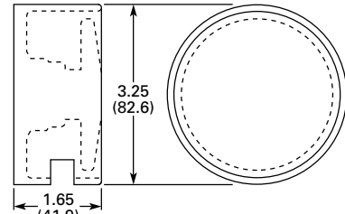
Protecting Shroud for Jumbo Mushroom Head Button Catalog No. 10250TA56
