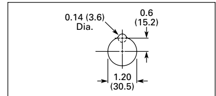
Figure 47-111. Drilling Dimensions in Inches (mm)
