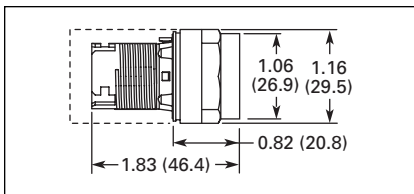
Figure 47-35. EM22 Series Illuminated Flush Operator
