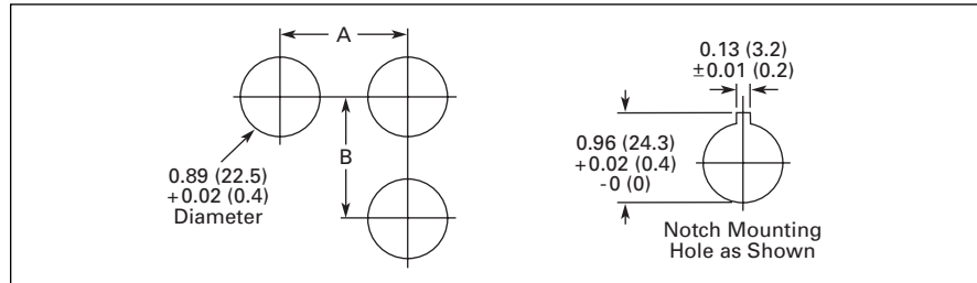
Figure 47-30. E22 Series Non-illuminated Flush Operator
