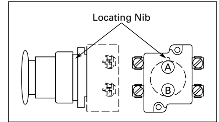
Figure 47-117. Contact Circuit Locations
