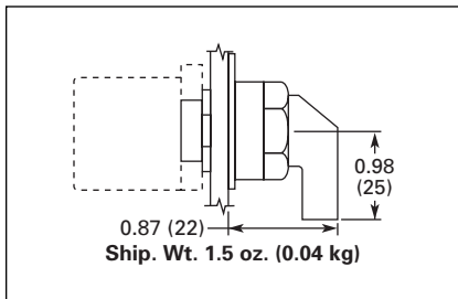
Figure 47-56. E22/EM22 Series 3-Position — 60° Throw — Lever
