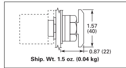
Figure 47-39. E22/EM22 Series 40 mm Dia. Push-Pull Button
