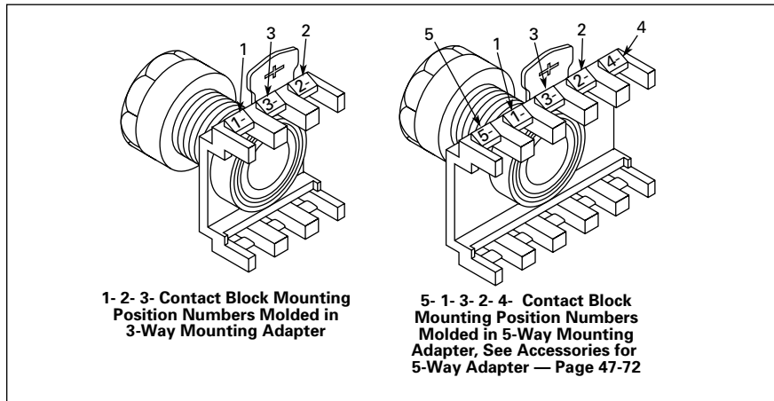
Figure 47-9. Contact Block Mounting
