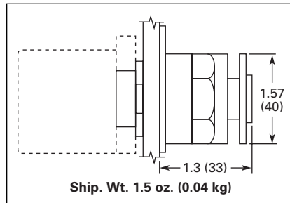
Figure 47-47. E22/EM22 Series 3-Position 40 mm Dia. Push-Pull Pushbutton (Spring Return to Center from Pulled Position)
