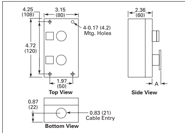
Figure 47-3. Two-Element — Approximate Dimensions in Inches (mm)
