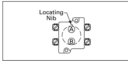
Figure 47-96. Mounting Location
