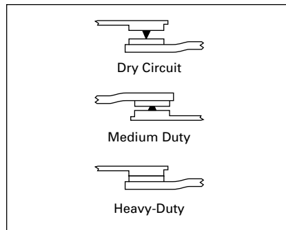
Figure 47-83. Reliability Nibs
