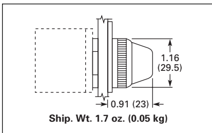
Figure 47-44. E22 Series 25 mm Dia. Glass Lens
