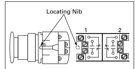
Figure 47-138. Locating Nibs
