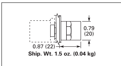
Figure 47-58. E22/EM22 Series 3-Position — 60° Throw — Knob
