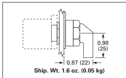
Figure 47-62. E22 Series 2-Position — 60° Throw — Lever
