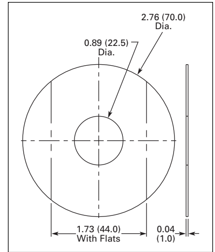
Figure 47-71. Joystick Nameplate Dimensions — Approximate Dimensions in Inches (mm)
