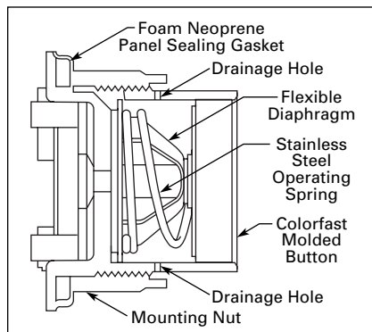
Figure 47-137. Diaphragm Seal
