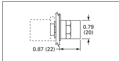
Figure 47-61. E22 Series 3-Position — 45° Throw — Knob
