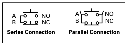
Figure 47-103. Series and Parallel Connection
