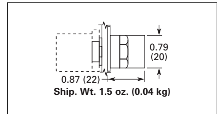
Figure 47-65. EM22 Series — 60° Throw — Knob
