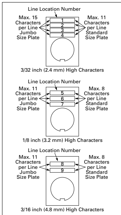
Figure 47-14. Aluminum and Plastic Legend Plates
