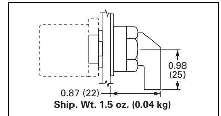
Figure 47-51. E22 Series 2-Position — 45° Throw — Lever
