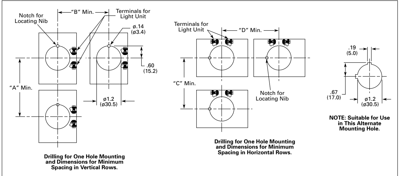
Figure 47-146. Panel Spacing and Drilling Drawings
