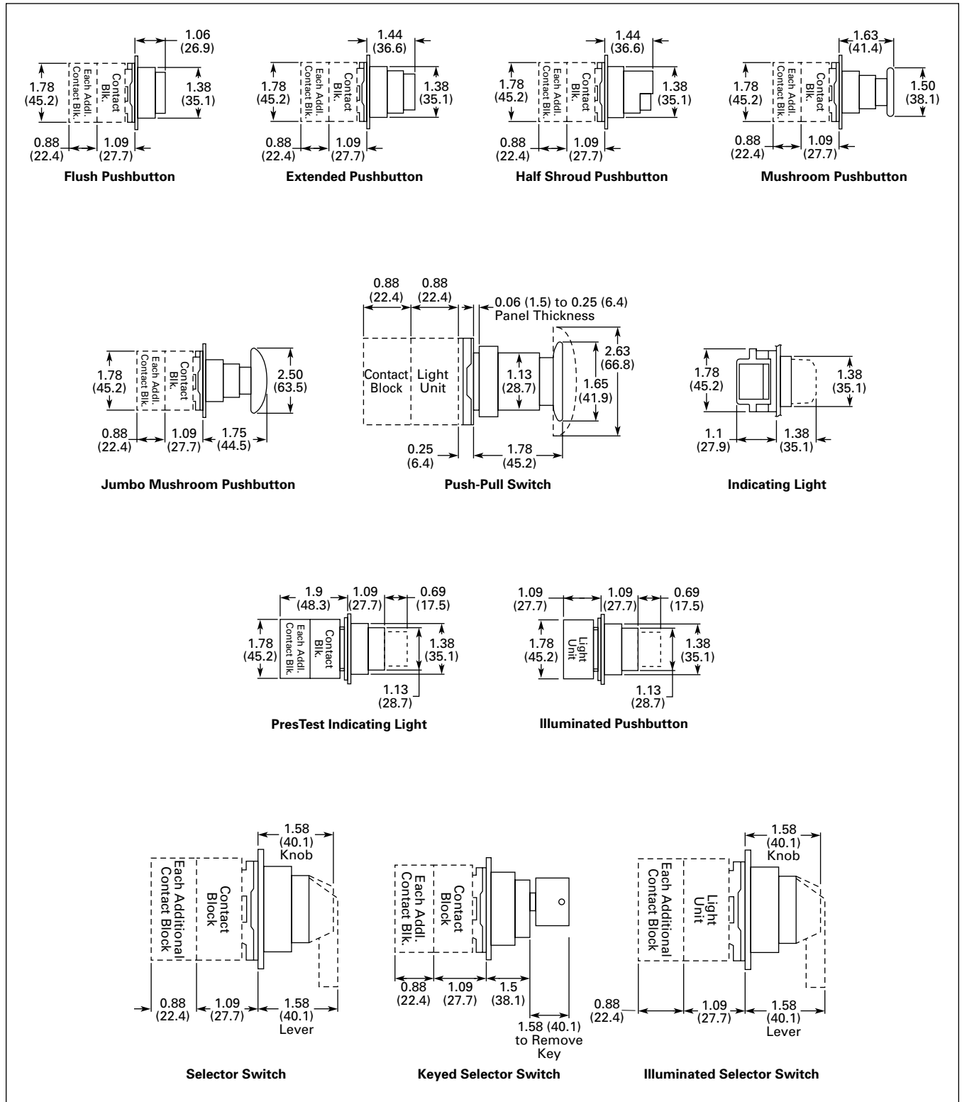
Figure 47-127. Approximate Dimensions in Inches (mm)
