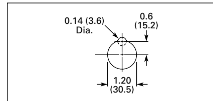
Figure 47-126. Drilling Dimensions in Inches (mm)
