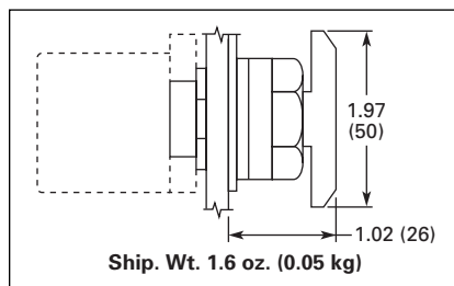
Figure 47-26. E22/EM22 Series 50 mm Dia. Mushroom Head Button
