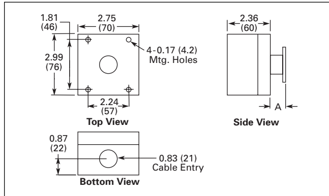
Figure 47-2. One-Element — Approximate Dimensions in Inches (mm)
