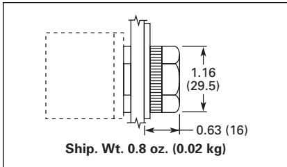
Figure 47-42. E22/EM22 Series 25 mm Dia. Standard Lens
