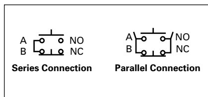
Figure 47-99. Series and Parallel Connections
