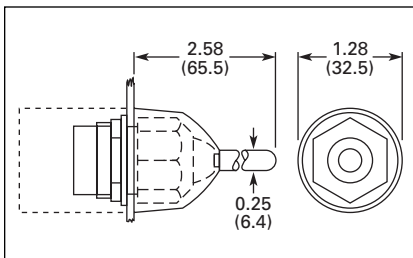
Figure 47-69. Wobble Stick Operator
