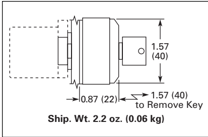
Figure 47-41. E22/EM22 Series 40 mm Dia. Key Release Button
