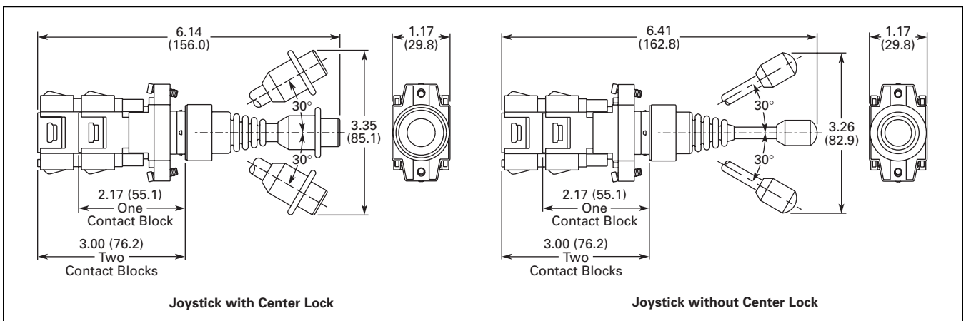
Figure 47-72. Joystick Operator Dimensions — Approximate Dimensions in Inches (mm)
