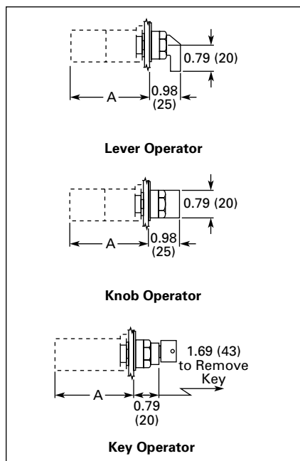
Figure 47-19. Approximate Dimensions in Inches (mm)
