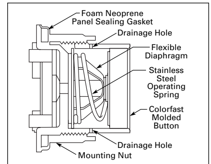
Figure 47-84. Diaphragm Seal
