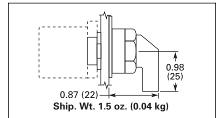
Figure 47-52. E22 Series 3-Position — 45° Throw — Lever
