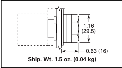
Figure 47-21. E22/EM22 Series 25 mm Dia. Flush Button
