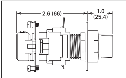
Figure 47-67. Potentiometer with Knob Operator
