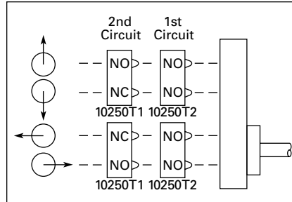
Figure 47-95. Example Contact Blocks and Locations
