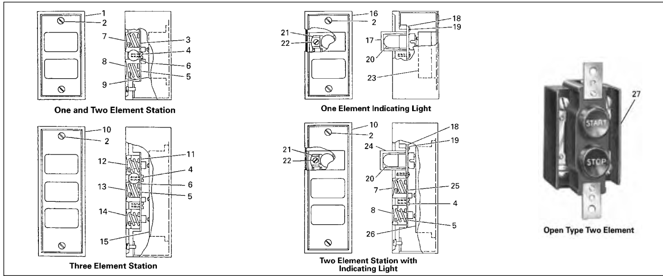
Figure 47-7. Type N Renewal Parts
