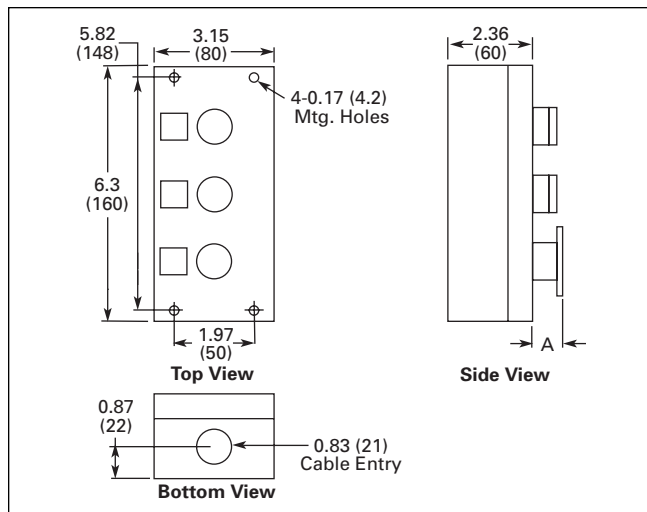
Figure 47-4. Three-Element — Approximate Dimensions in Inches (mm)
