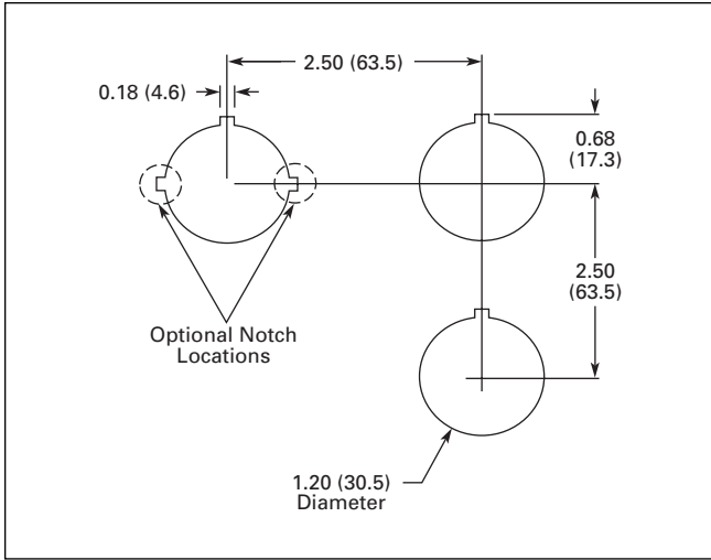
Figure 47-135. Mounting Matrix and Minimum Panel Spacing Requirements in Inches (mm)
