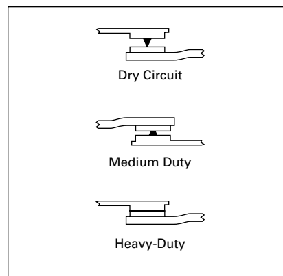
Figure 47-75. Reliability Nibs
