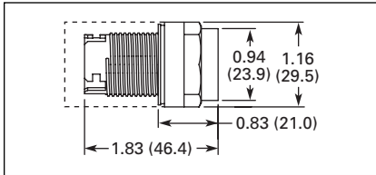
Figure 47-31. E22 Series Non-illuminated Extended Operator
