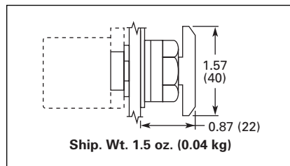
Figure 47-38. E22/EM22 Series 40 mm Dia. Twist-to-Release Button
