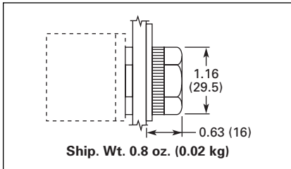
Figure 47-43. E22/EM22 Series 25 mm Dia. Lens Insert Version
