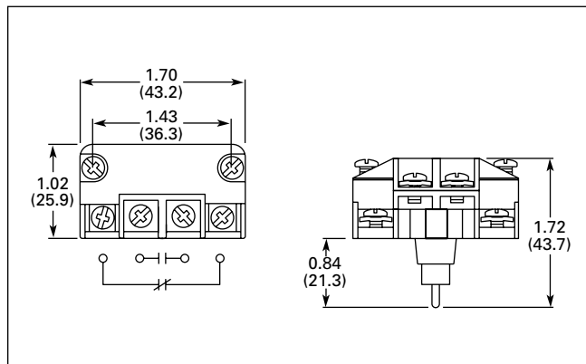
Figure 47-143. Contact Block
