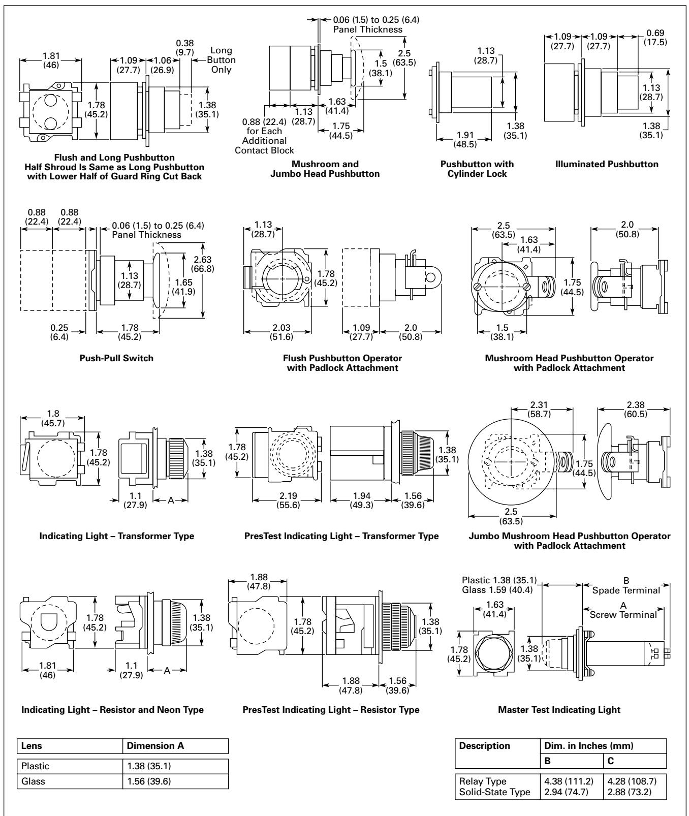
Figure 47-112. Approximate Dimensions in Inches (mm)
