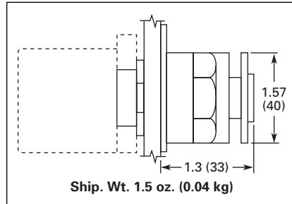
Figure 47-45. E22/EM22 Series 2-Position 40 mm Dia. Button (Maintained)
