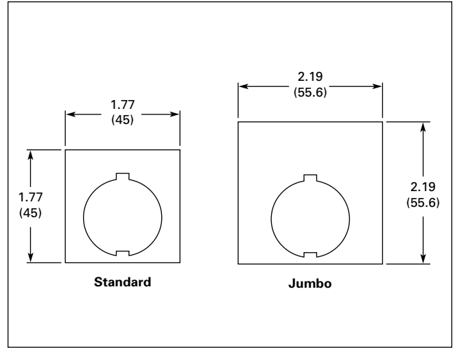
Figure 47-136. Legend Plates — Approximate Dimensions in Inches (mm)
