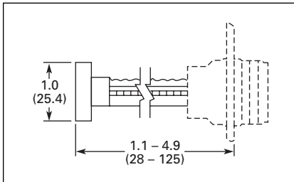
Figure 47-68. Flush Pushbutton Operator with Mechanical Push Rod
