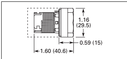
Figure 47-33. EM22 Series Non-illuminated Flush Operator
