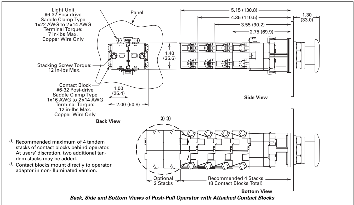
Figure 47-132. Illuminated and Non-illuminated Flat Head MRH Push-Pull Operators — Approximate Dimensions in Inches (mm)
