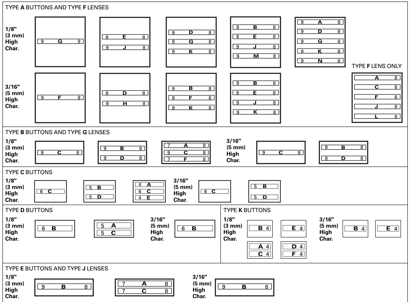
Figure 47-78. Legend Locations
