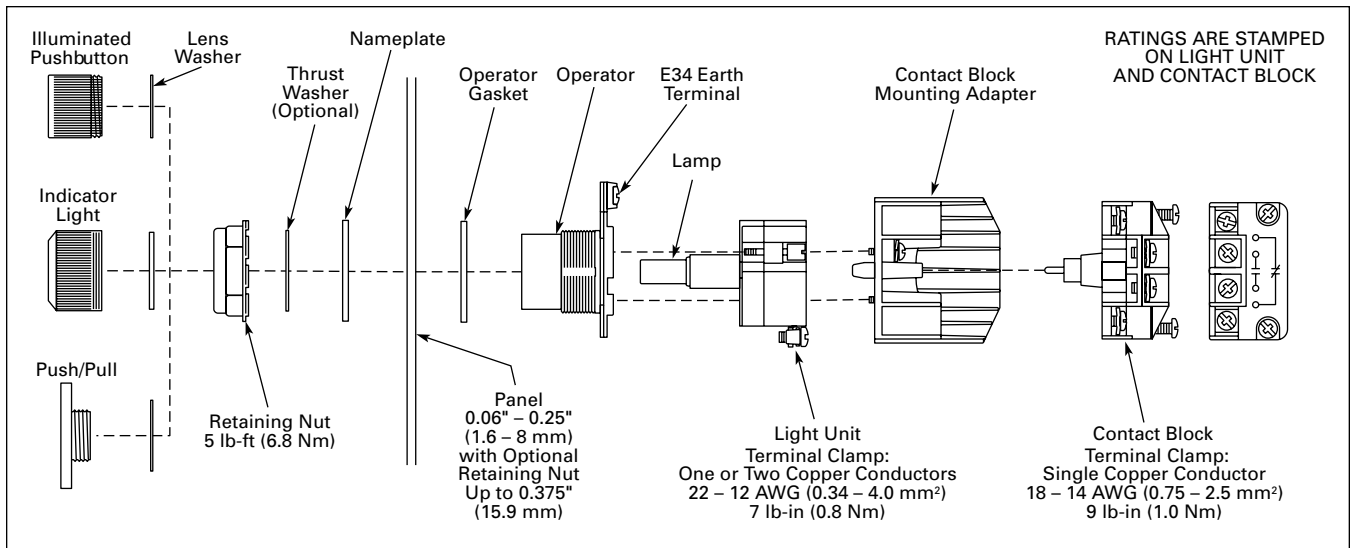
Figure 47-147. Operator Assembly
