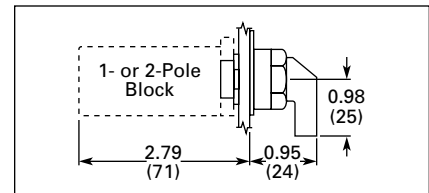
Figure 47-66. Rotary Cam Selector Switch For each additional (1- or 2-pole) block add 0.47" (12 mm).
