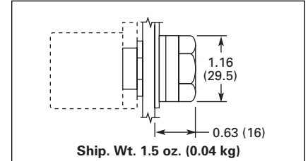
Figure 47-27. E22/EM22 Series 25 mm Dia. Flush Lens
