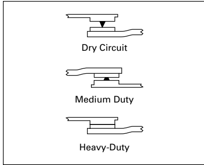
Figure 47-115. Reliability Nibs
