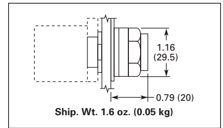
Figure 47-28. E22/EM22 Series 25 mm Dia. Extended Lens
