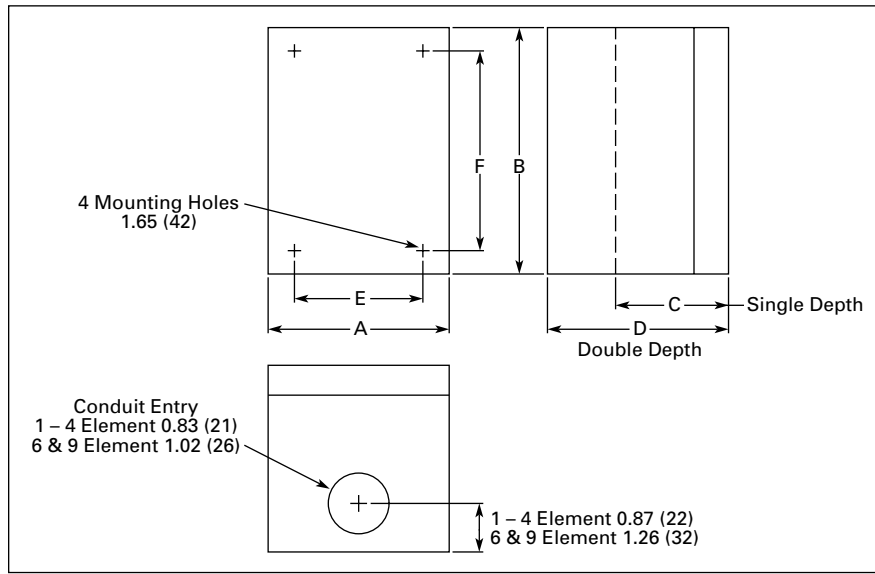
Figure 47-20. Enclosure Dimensions in Inches (mm)
