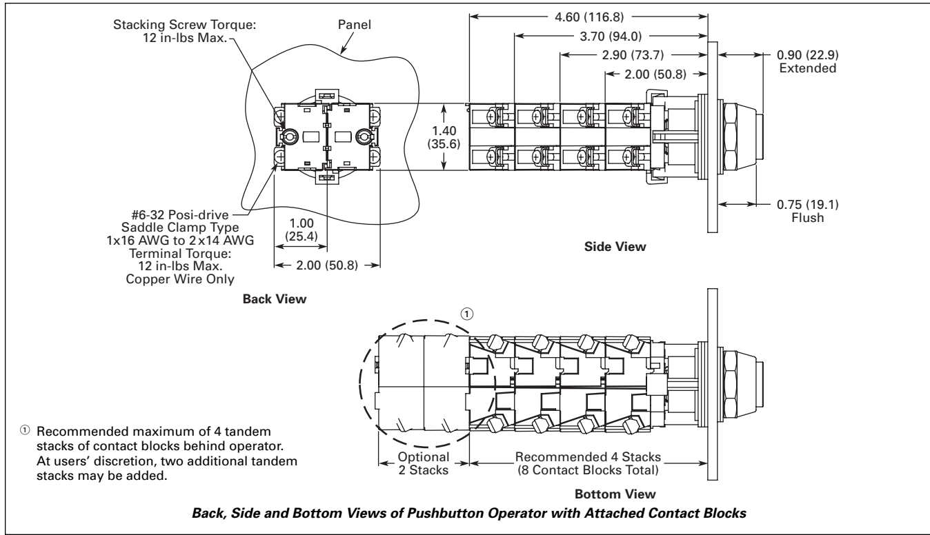
Figure 47-129. Momentary Pushbuttons — Non-illuminated — Approximate Dimensions in Inches (mm)
