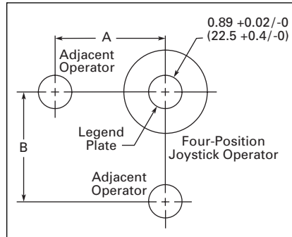
Figure 47-70. Joystick Mounting — Approximate Dimensions in Inches (mm)
