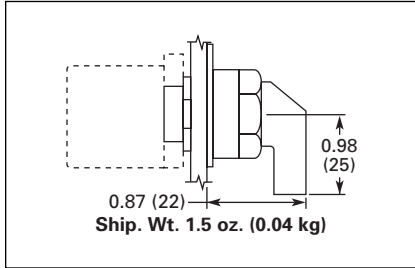
Figure 47-55. E22/EM22 Series 2-Position — 60° Throw — Lever
