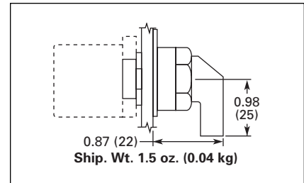
Figure 47-64. EM22 Series — 60° Throw — Lever
