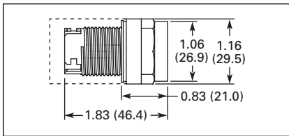
Figure 47-32. E22 Series Illuminated Flush Operator
