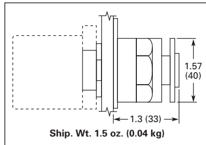
Figure 47-46. E22/EM22 Series 3-Position 40 mm Dia. Button (Spring Return to Center)
