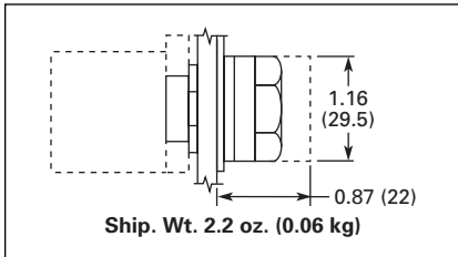
Figure 47-23. E22/EM22 Series 25 mm Dia. with Full Shroud
