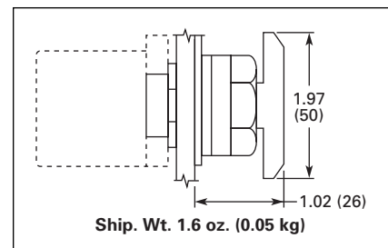
Figure 47-40. E22/EM22 Series 50 mm Dia. Push-Pull Button
