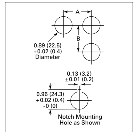
Figure 47-10. Minimum Spacing in Inches (mm)
