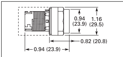
Figure 47-34. EM22 Series Non-illuminated Extended Operator
