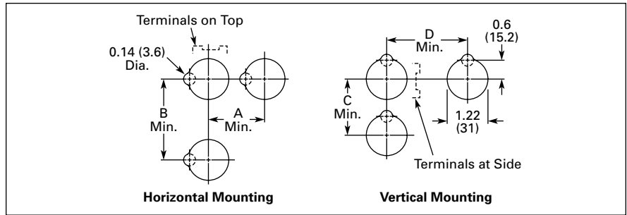
Figure 47-110. Mounting Options in Inches (mm)
