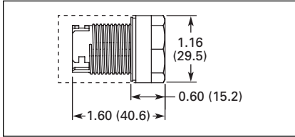
Figure 47-30. E22 Series Non-illuminated Flush Operator
