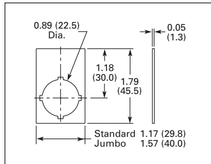
Figure 47-36. Push-Push Nameplate Dimensions
