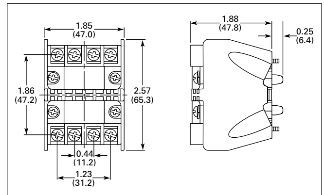
Figure 47-144. Mounting Adapter
