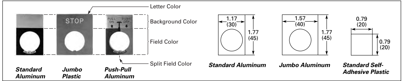
Figure 47-12. Color Diagram and Approximate Dimensions in Inches (mm)
