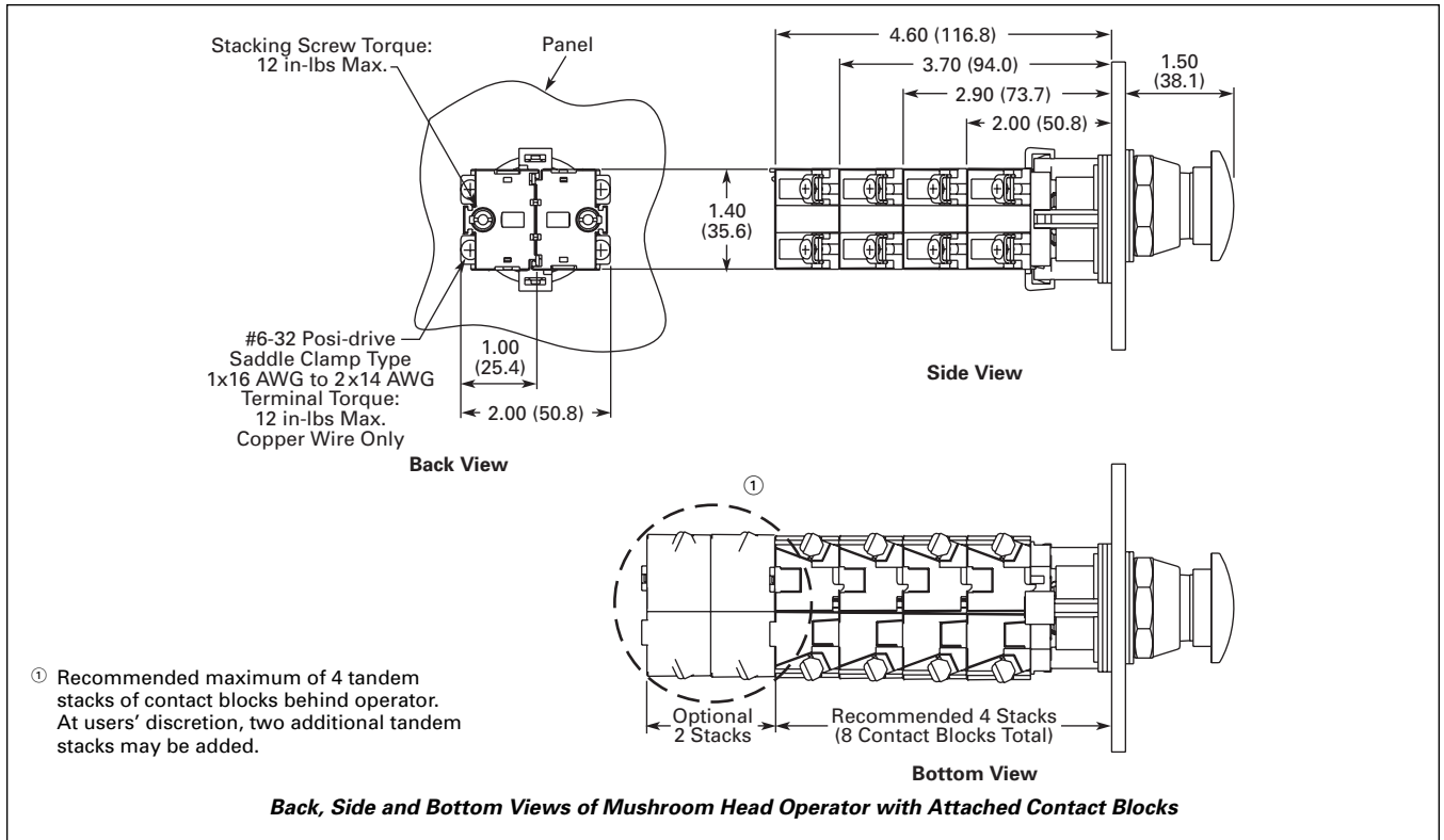
Figure 47-131. Mushroom Head Pushbuttons and Round Head MRH Push-Pull Operators — Approximate Dimensions in Inches (mm)
