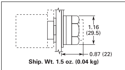
Figure 47-22. E22/EM22 Series 25 mm Dia. Extended Button
