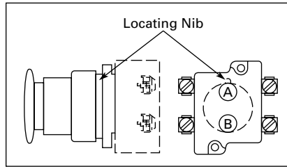
Figure 47-85. Contact Circuit Locations
