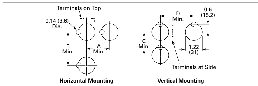
Figure 47-125. Mounting Options in Inches (mm)
