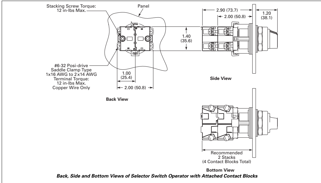
Figure 47-134. Selector Switches— Approximate Dimensions in Inches (mm)
