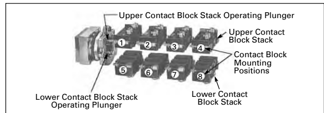
Figure 47-76. Mounting Positions
