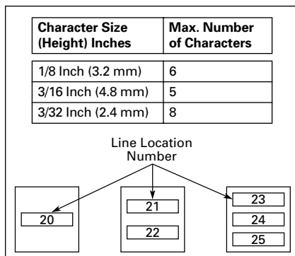
Figure 47-15. Enclosure Legend Plates — Self-Adhesive
