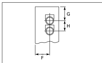
Figure 47-123. Spacing Increments for Enclosures
