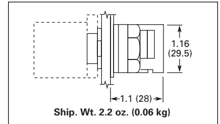
Figure 47-29. E22/EM22 Series 25 mm Dia. Extended Lens with Shroud
