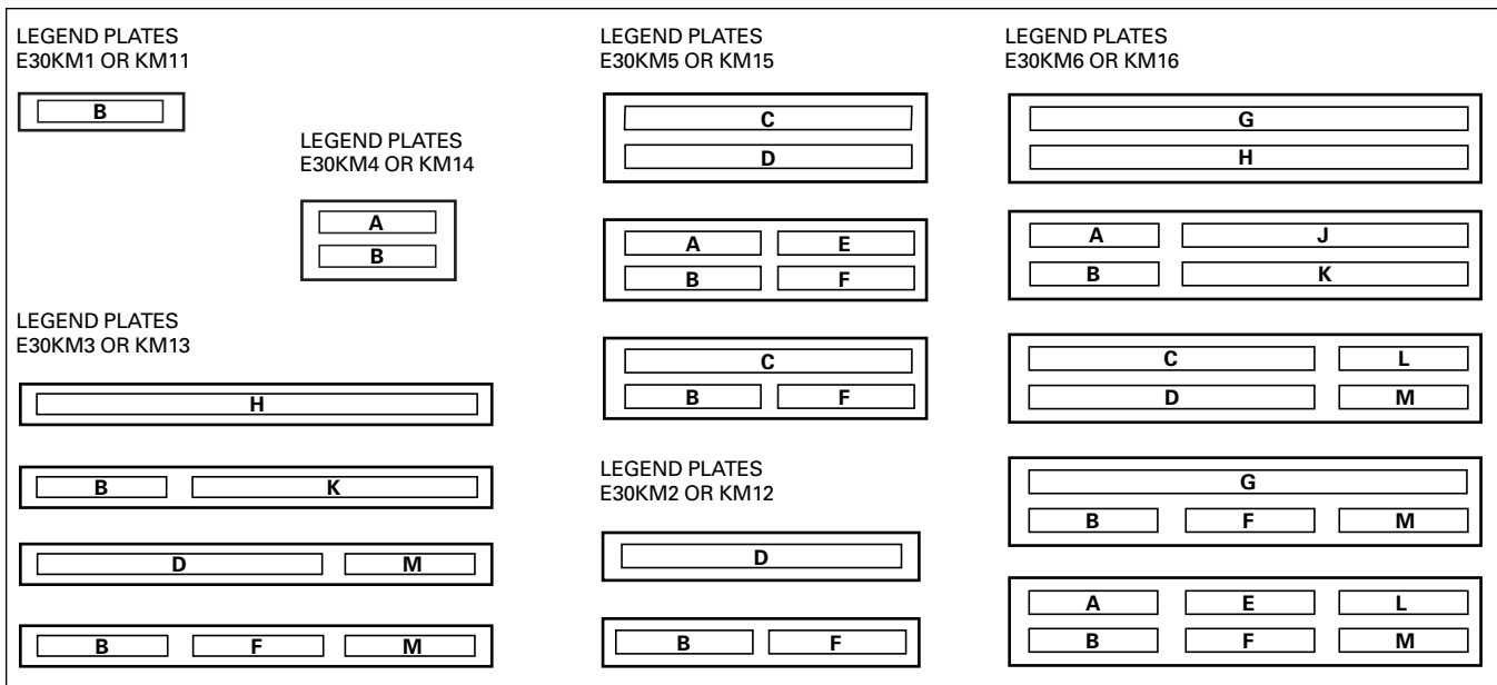
Figure 47-79. Legend Arrangements and Legend Locations
