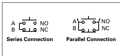
Figure 47-97. Series and Parallel Connections
