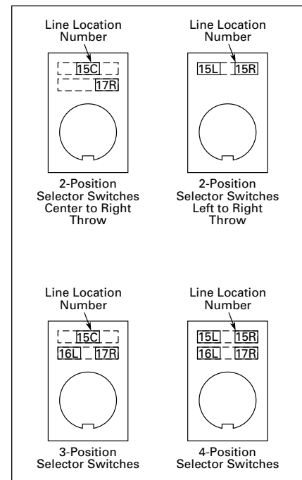
Figure 47-18. Selector Switch Legend Plates
