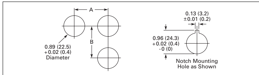
Figure 47-73. Minimum Spacing in Inches (mm)
