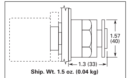
Figure 47-50. E22/EM22 Series 3-Position 40 mm Dia. Push-Pull Pushbutton (Spring Return to Center from Pulled Position)
