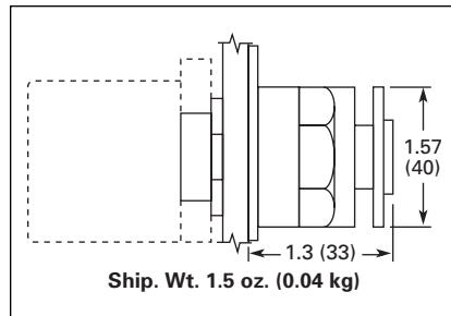
Figure 47-48. E22/EM22 Series 2-Position 40 mm Dia. Lens (Maintained)
