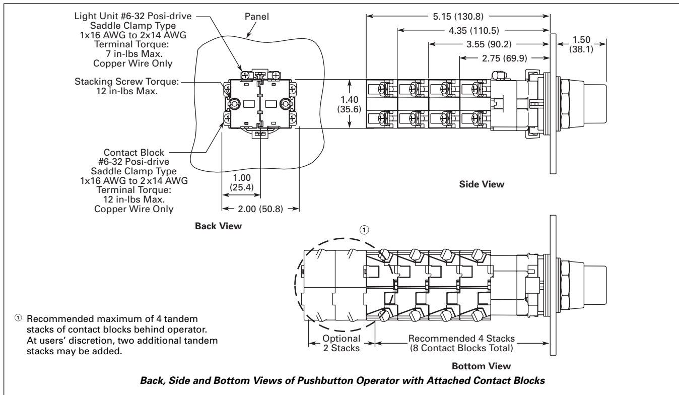
Figure 47-130. Illuminated Pushbuttons — Approximate Dimensions in Inches (mm)
