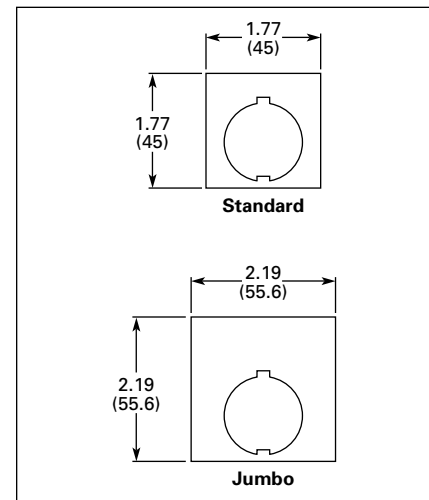
Figure 47-121. Approximate Dimensions in Inches (mm)
