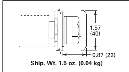
Figure 47-25. E22/EM22 Series 40 mm Dia. Mushroom Head Button
