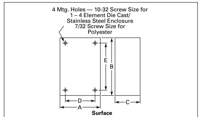
Figure 47-5. Approximate Enclosure Dimensions
