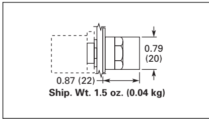
Figure 47-54. E22 Series 3-Position — 45° Throw — Knob
