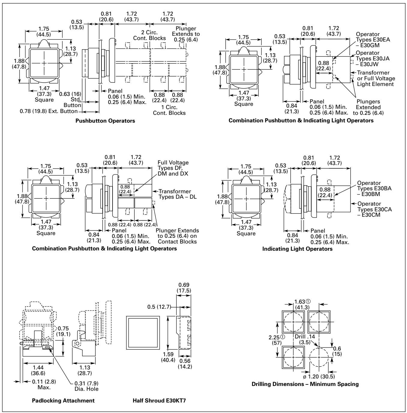
Figure 47-82. Approximate Dimensions in Inches (mm)
