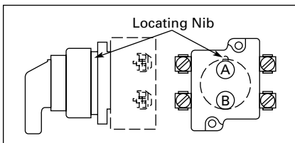
Figure 47-87. Contact Circuit Locations
