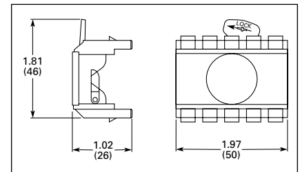
Figure 47-11. Overall Dimensions in Inches (mm)
