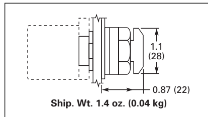
Figure 47-37. E22/EM22 Series 28 mm Diameter Twist-to-Release Button
