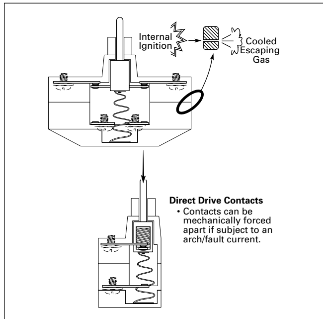
Figure 47-148. Factory Sealed Contact Blocks
