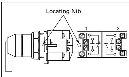
Figure 47-140. Contact Circuit Locations
